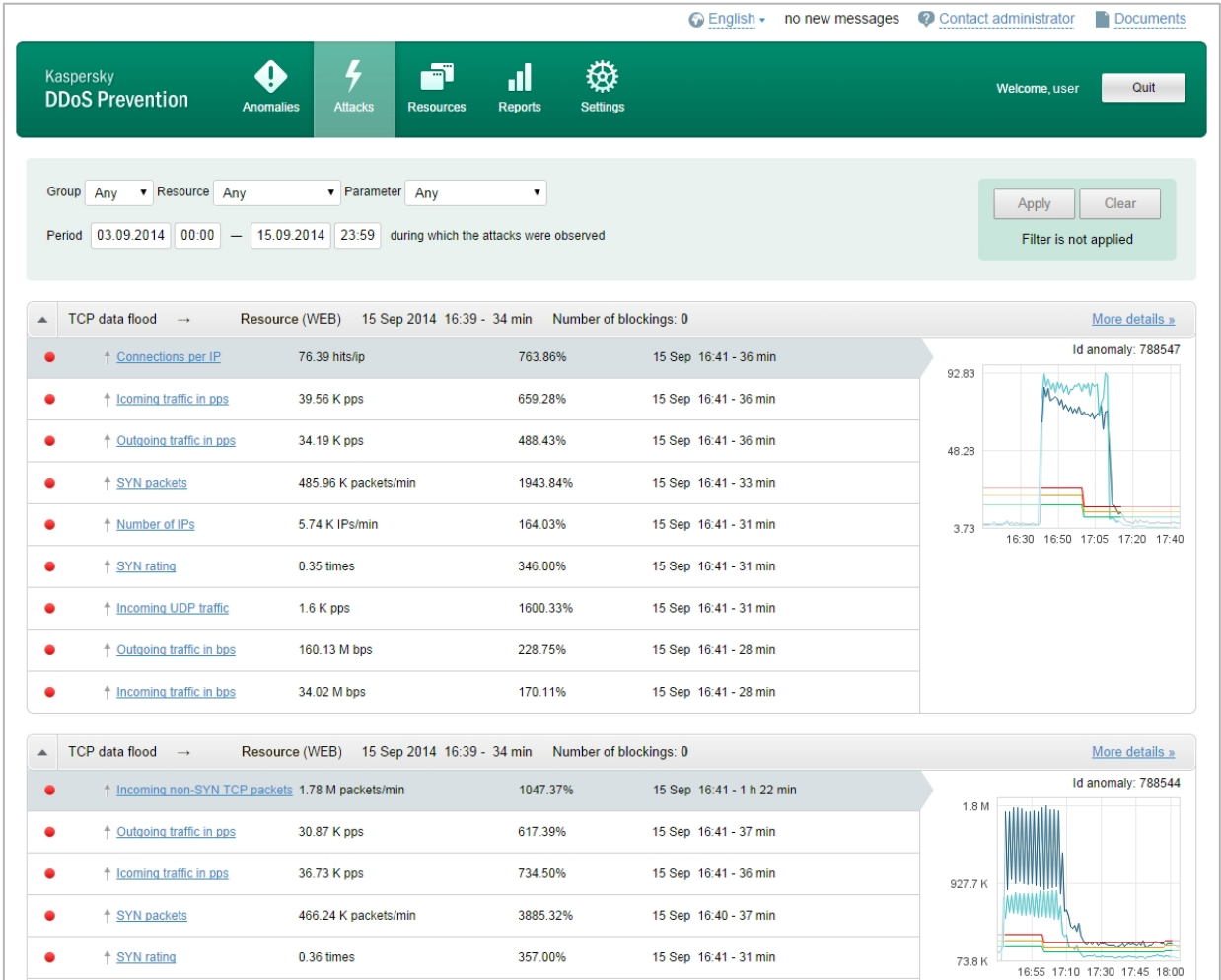
Figure 3. Screenshot of the client's interface
